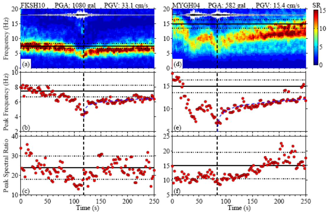
Fig. 3. (a) Color-coded surface/borehole spectral ratios plotted against time for the station FKSH10. The x-axis shows the time since the beginning of the recording, and the y-axis shows the frequency. The spectral ratio values are color-coded with red being high and blue being low. The vertical dashed lines indicate the time when the highest PGA value is recorded. The horizontal solid and dotted lines show the reference value and uncertainties of the peak frequency obtained by averaging all the spectral ratios for the windows before the P-arrivals of all the earthquakes between 2011/01/01 and 2011/03/28. The white and black traces on the top show the waveforms of the surface and borehole recordings, respectively. (b) Measured peak frequencies from (a). The horizontal and vertical lines are the same as in (a). The blue dashed curve shows the least-squares logarithmic fitting of the peak frequencies after the highest PGA. (c) Measured peak spectral ratios from (a). The horizontal solid and dotted lines show the reference value and uncertainties of the peak spectral ratio obtained by averaging all the spectral ratios for the windows before the P-arrivals of all the earthquakes between 2011/01/01 and 2011/03/28. (d-f) Similar plots as (a-c) for the station MYGH04.
