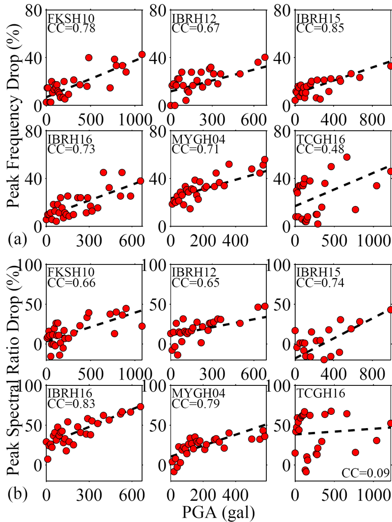
Fig. 4. (a) Calculated percentage drop of peak frequencies plotted against PGA at the six stations during the Tohoku main shock. The black dashed line shows the least-squares fitting of the data. Station names and correlation coefficient values are marked on the top-left corner of each panel. (b) Similar fig. as (a) for the percentage drop of the peak spectral ratios.
