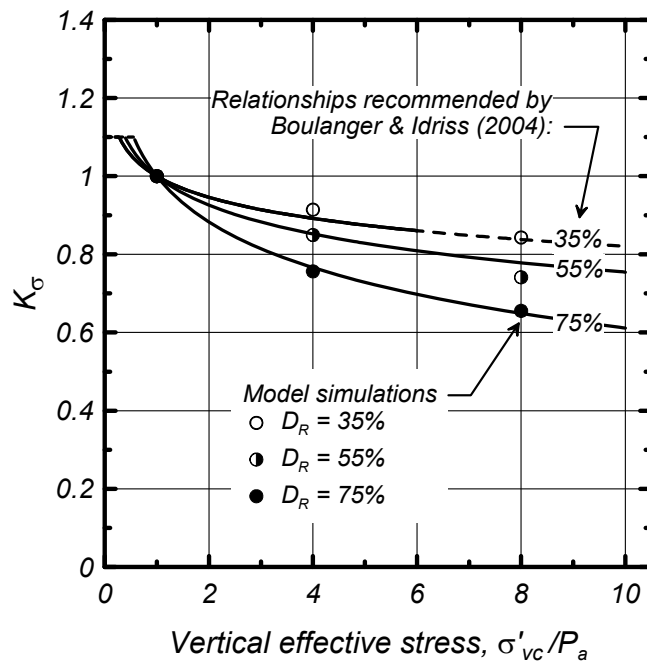
Fig. 5. Comparison of K_\sigma ratios from simulations versus relationships by Boulanger and Idriss (2004).
